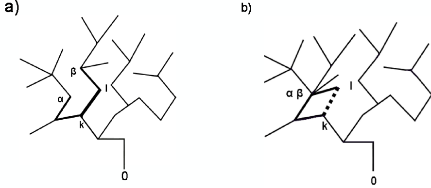
Figure 1: Figure 1a) represents an mt in (N_0, C) . The most expensive arc in the path that connects \alpha and \beta is (k, l) . In Figure 1b) nodes \alpha and \beta join and the most expensive arc is removed. The resulting tree is a mt in the reduced problem.
