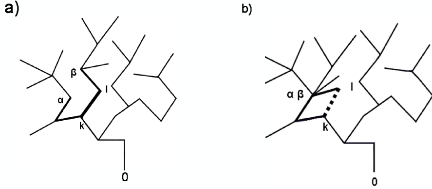
Figure 1: Figure 1a) represents an mt in (N_0, C) . The most expensive arc in the path that connects \alpha and \beta is (k, l) . In Figure 1b) nodes \alpha and \beta join and the most expensive arc is removed. The resulting tree is a mt in the reduced problem.
